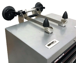
K4600-2 Glasstable with tilt function and vacuum suction cup with double lip ( for trolley )
